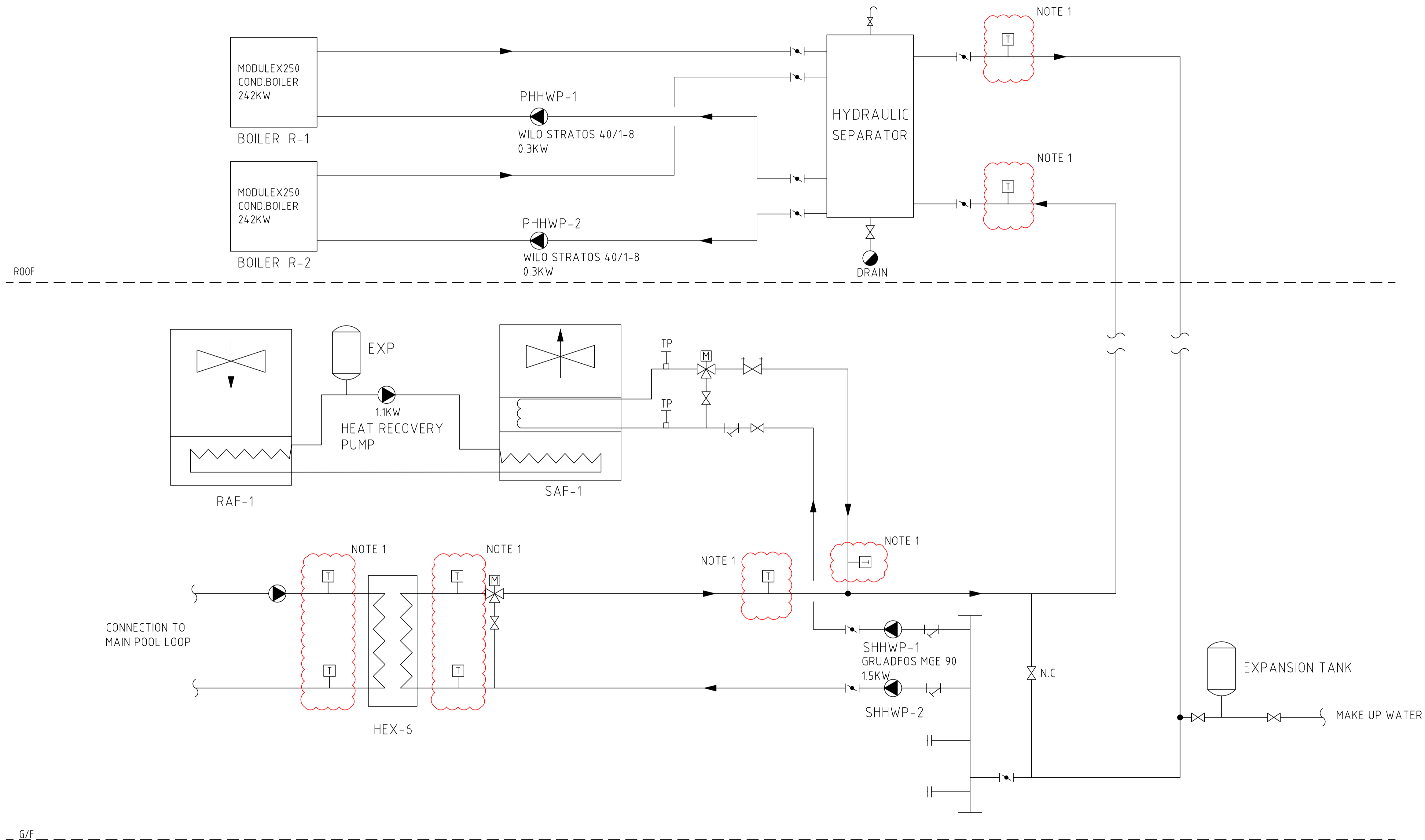
INDOOR HEATING HOT WATER SYSTEM SCHEMATIC NOT TO SCALE
