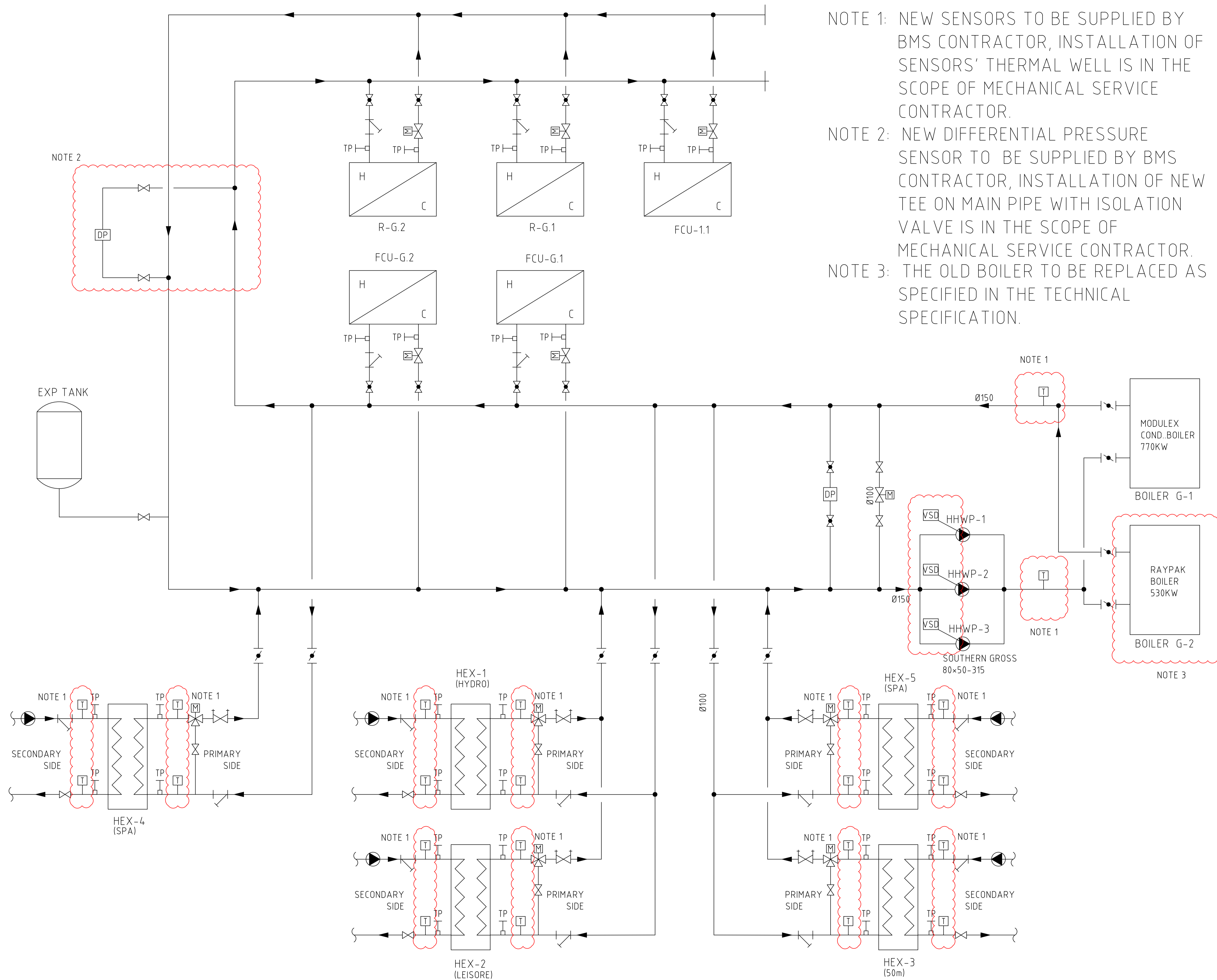
OUTDOOR HEATING HOT WATER SYSTEM SCHEMATIC NOT TO SCALE
